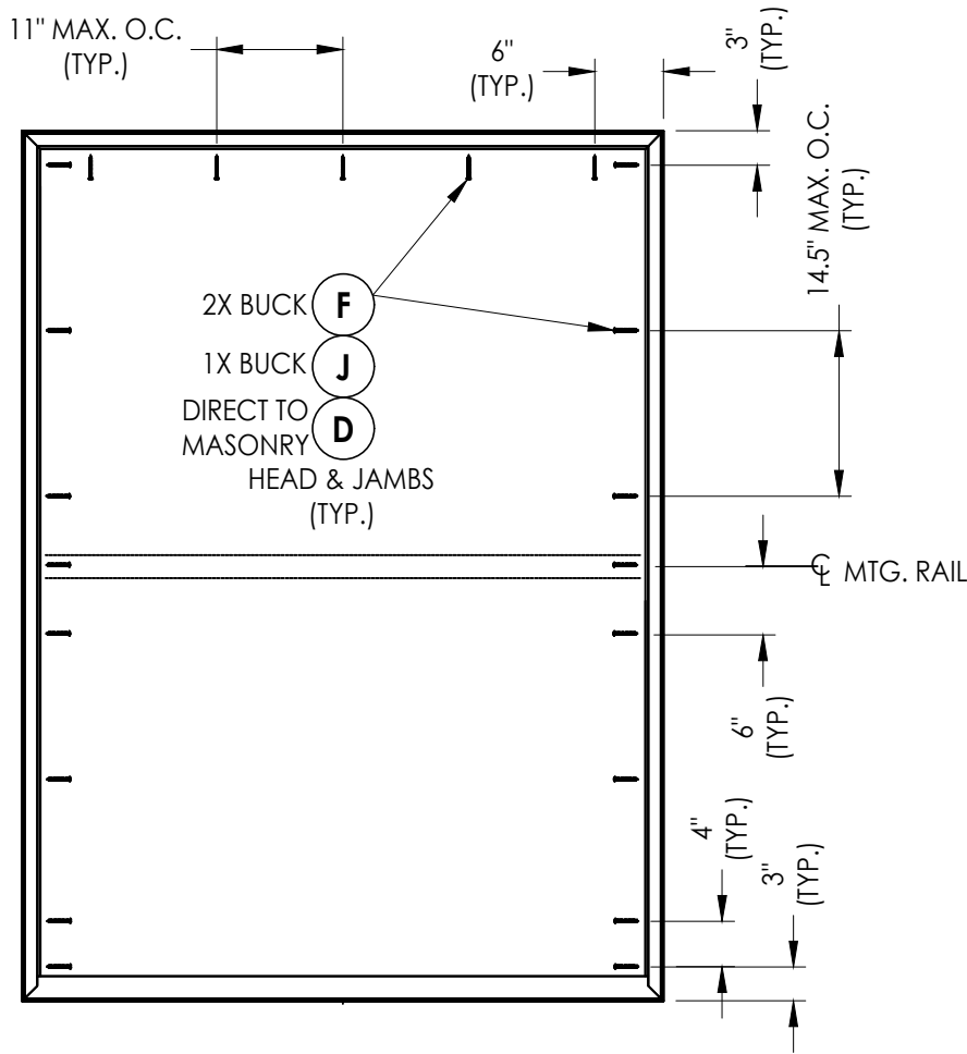
FRAME ANCHORING 56" X 84" MAX. FRAME SIZE
