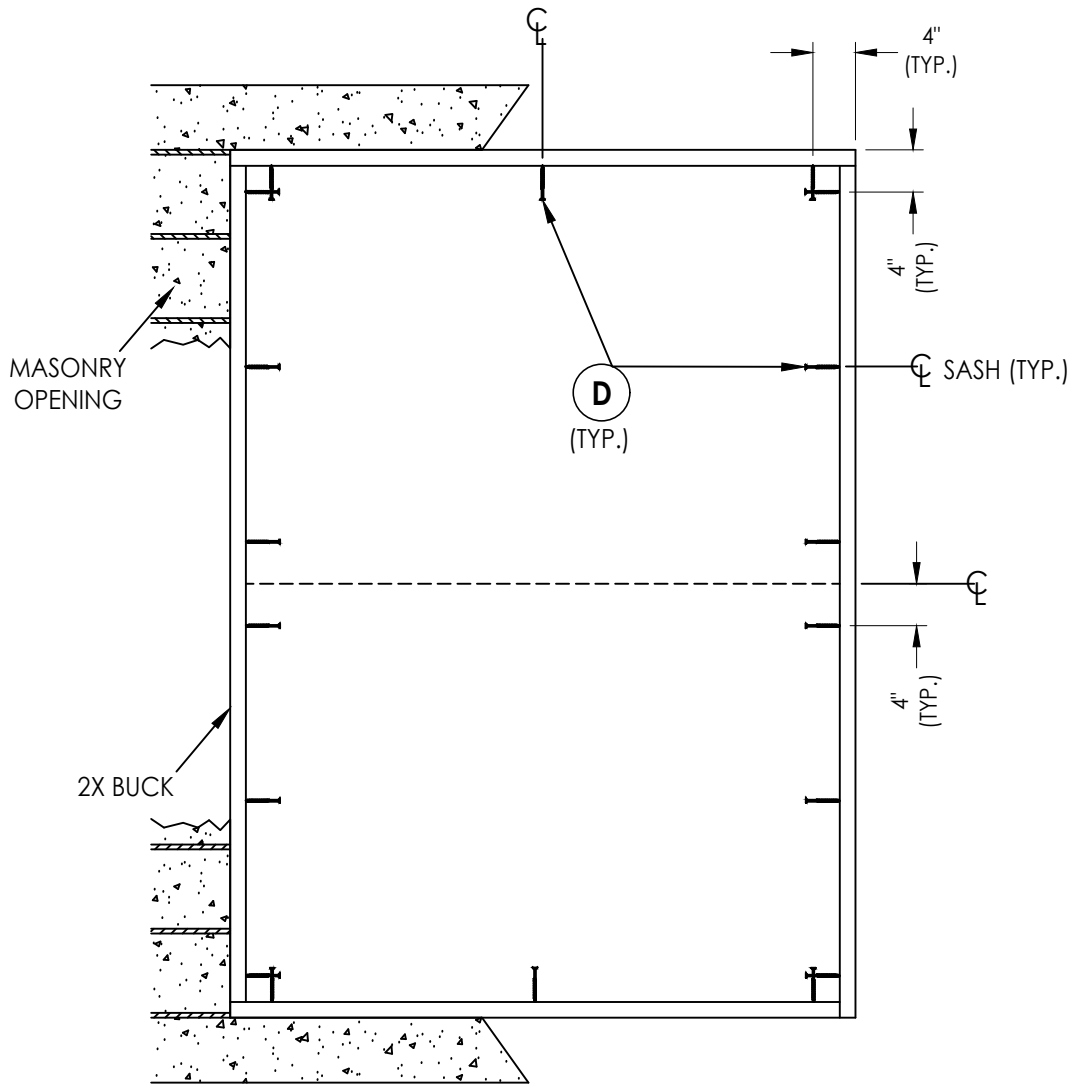
BUCK ANCHORING 56" X 84" MAX. FRAME SIZE
